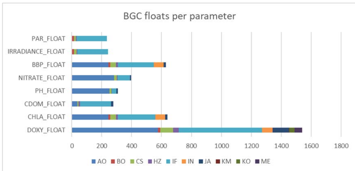
BGC-Argo floats distribution per parameter and DAC
